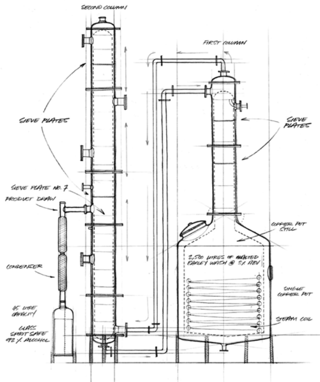
OUR UNIQUE FARADAY POT STILL
